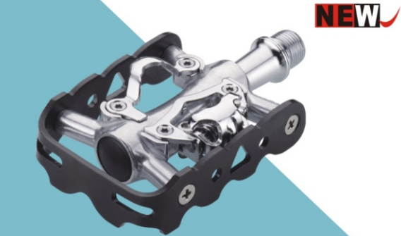
Model:HF-707 DUAL FUNCTION Body: Aluminum Barrel polished polished/Anodized Bearing:DU bearing or Sealed Axle:CR-MO/Boron Size:101x63mm Weight:Ball typr 328g/pr
