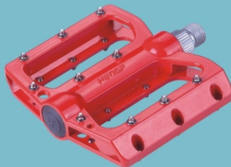
Model:HF-882S MTB/BMX Body:Aluminum Extruded/CNC machined Bearing:Sealed Axle: CR-MO/Boron Size:110x105mm Weight:Ball typr 426g/pr
